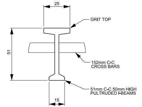
DETAIL C
