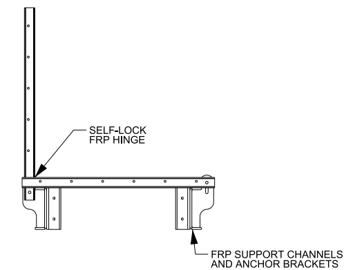
SIDE VIEW OF GRATING IN OPEN POSITION
