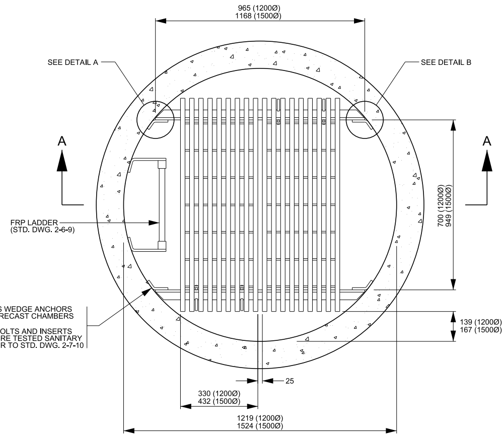
PLAN VIEW DETAIL OF GRATING AND BOLT-ON SUPPORT
